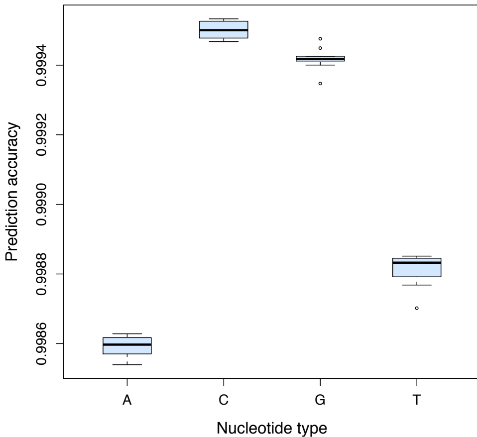
Figure 7: Variability of the prediction accuracy of HPCall. The obtained prediction accuracies are very stable among the different random samples of training data. The standard deviations of the prediction accuracies range from 0.000024 (for nucleotide C) to 0.000047 (for nucleotide T).
