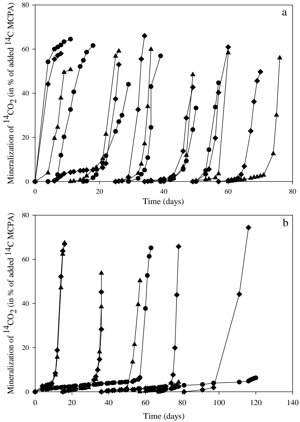
Figure S1. Mineralization of ^{14}\text{C} -ring labeled MCPA ( 0.1 \text{ mg L}^{-1} ) (a) ( 25 \text{ mg L}^{-1} ) (b) to \text{CO}_2 in successive enrichments. Different symbols represent different subcultures.
