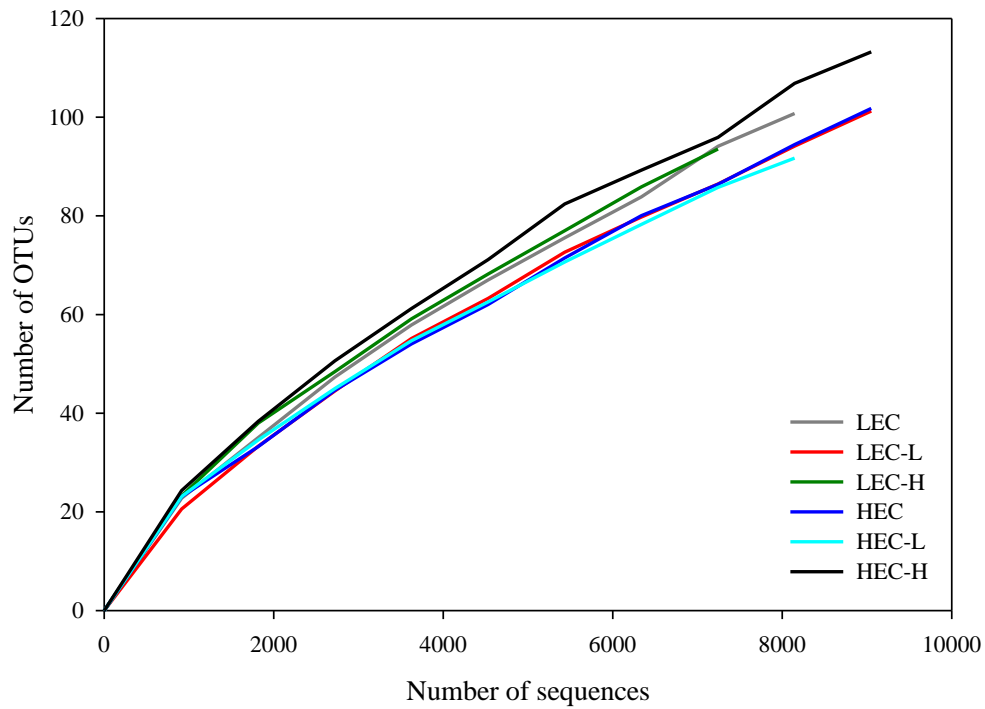
Figure S2. Rarefaction curves representing the relation between the number of sequences and the number of operational taxonomic units (OTUs) identified. The sequences were clustered and OTUs defined by 97% sequence identity using UCLUST, and reference sequences were picked using scripts in QIIME.
