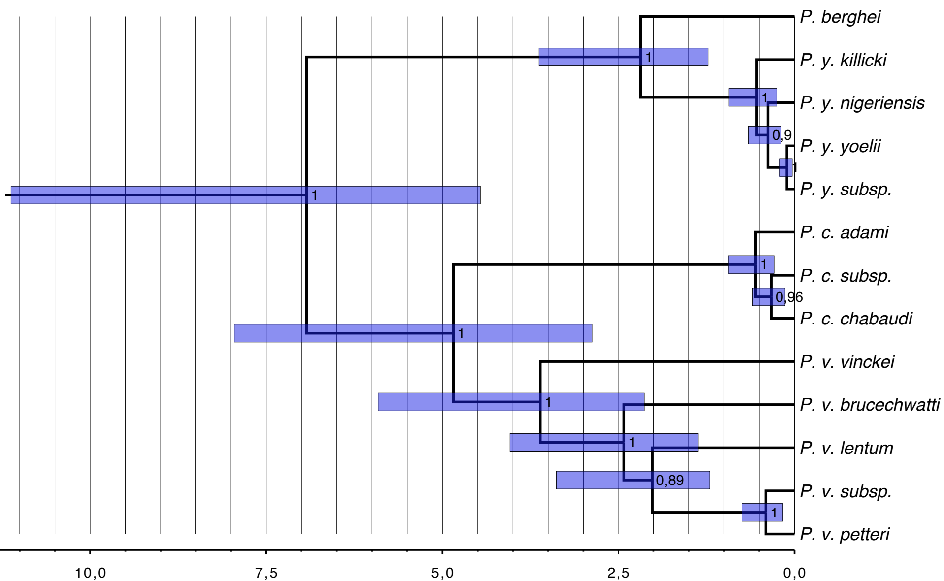
Additional File 11. Species tree inferred by *BEAST under the Pacheco2011-A calibration. Node labels are posterior probabilities and node bars represent 95% Highest Posterior Densities on the height of each node. Axis is in million years ago (Mya).
