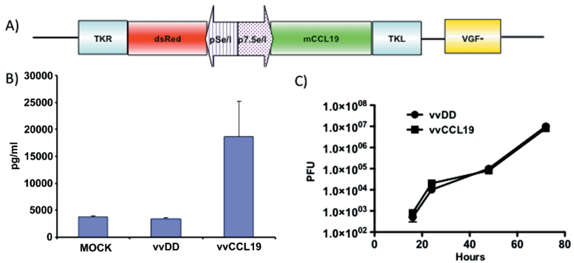
Figure W1. (A) Diagram displaying construction of vvCCL19 (TKR, thymidine kinase right-hand region; TKL, thymidine kinase left-hand region; VGF, vaccinia growth factor; pSe/L, synthetic early/late promoter; p7.5 E/L, 7.5 promoter early/late). (B) Production of CCL19 under different conditions (detected by ELISA in media 24 hours after infection of MC38 cell layer at MOI of 1.0). (C) Replication of vvDD and vvCCL19 in MC38 cells as determined by plaque assay on CV-1 cells (MOI of 1.0).
