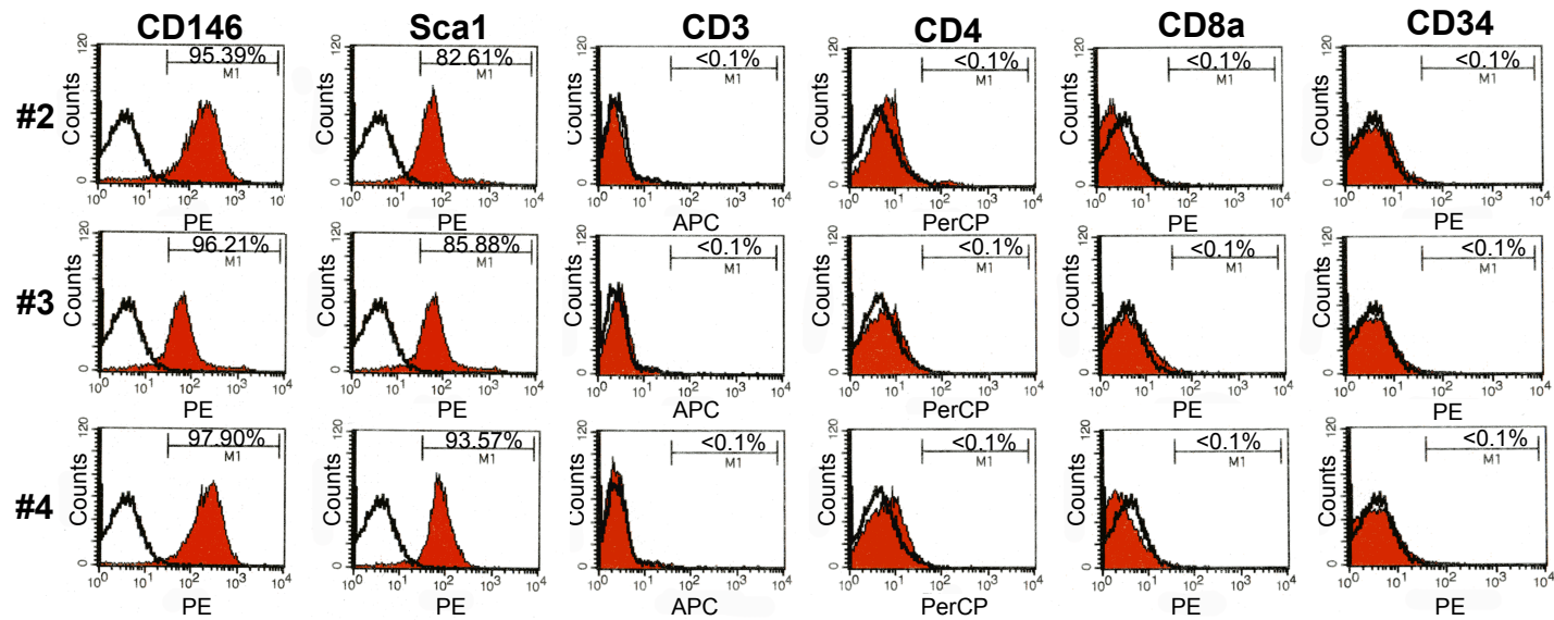
Figure S5. Flow cytometric analysis showed that IL-17 + MSCs (#2, #3, and #4) expressed stem cell markers CD146 and Sca1, but not hematopoietic markers CD34, CD3, CD4 and CD8a. Isotopic IgGs were used as negative control. The data are representative of three independent experiments.
