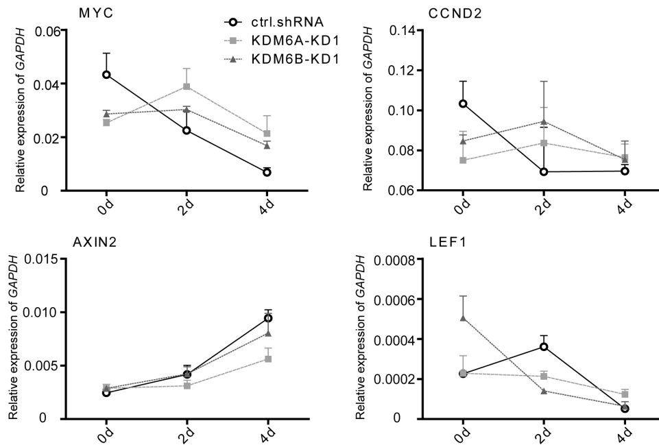
Supplemental Figure S7: KDM6A/KDM6B knockdown alters WNT target gene expression under definitive endoderm differentiation conditions. The expression levels of four genes of WNT signaling pathway MYC , CCND2 (also CYCLIN D2 ), AXIN2 and LEF1 were analyzed by RT-qPCR at different days during endoderm differentiation.
