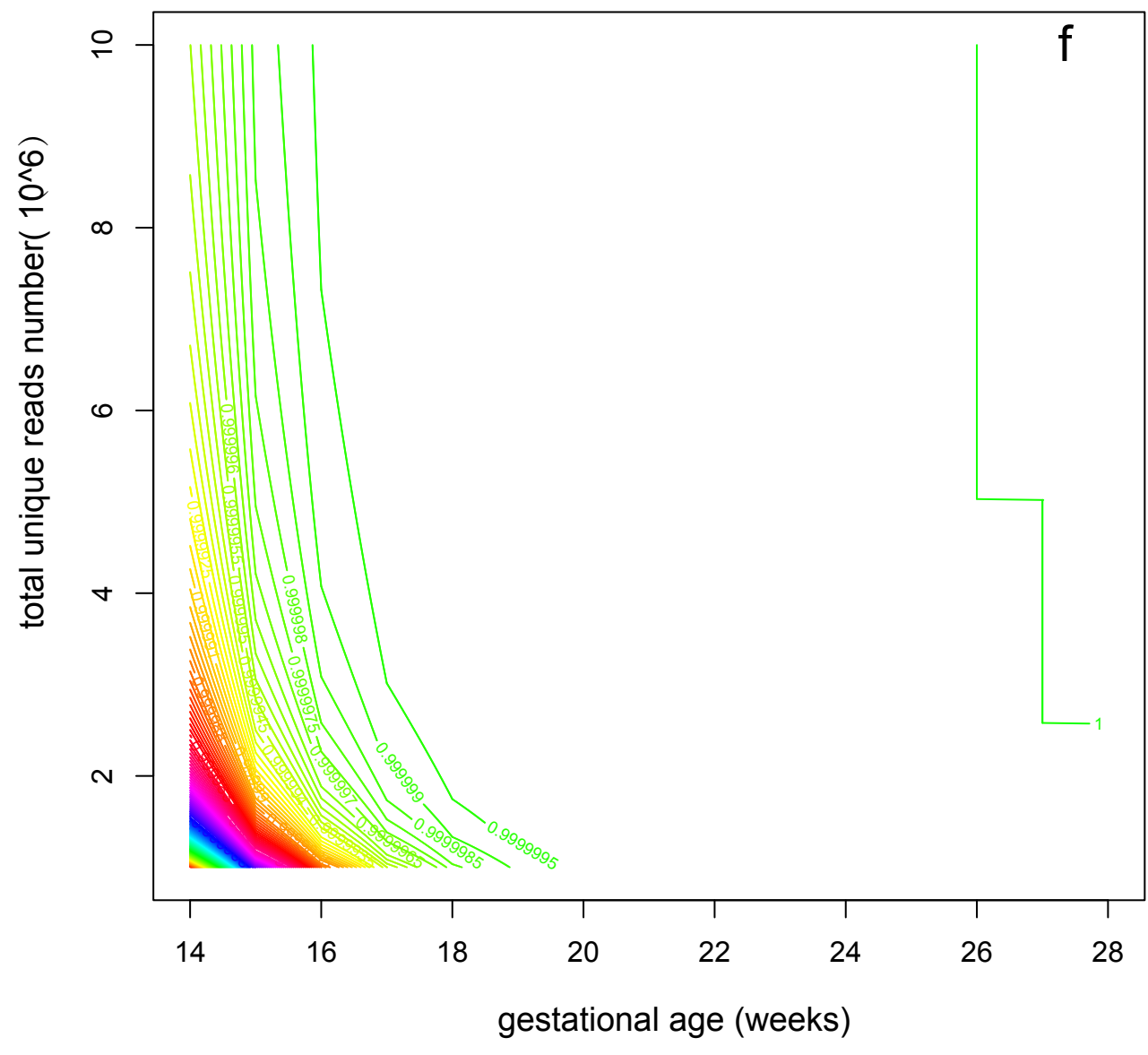
sensitivity of chr21 of male
