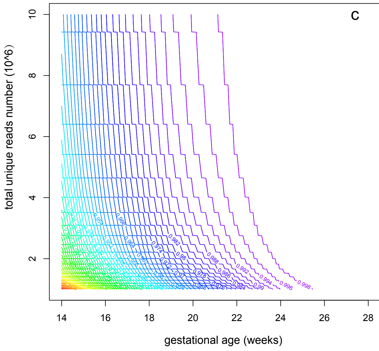
sensitivity of chr18 of female
