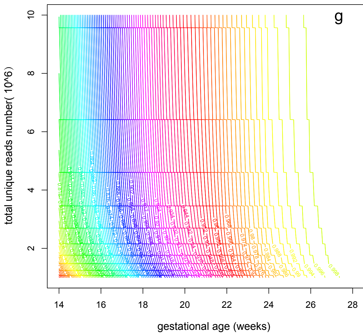
sensitivity of XXX or XO of chrX of female
