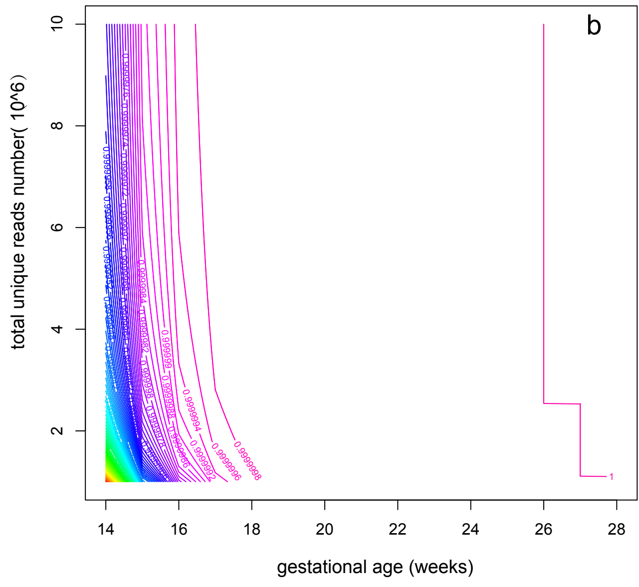
sensitivity of chr18 of male
