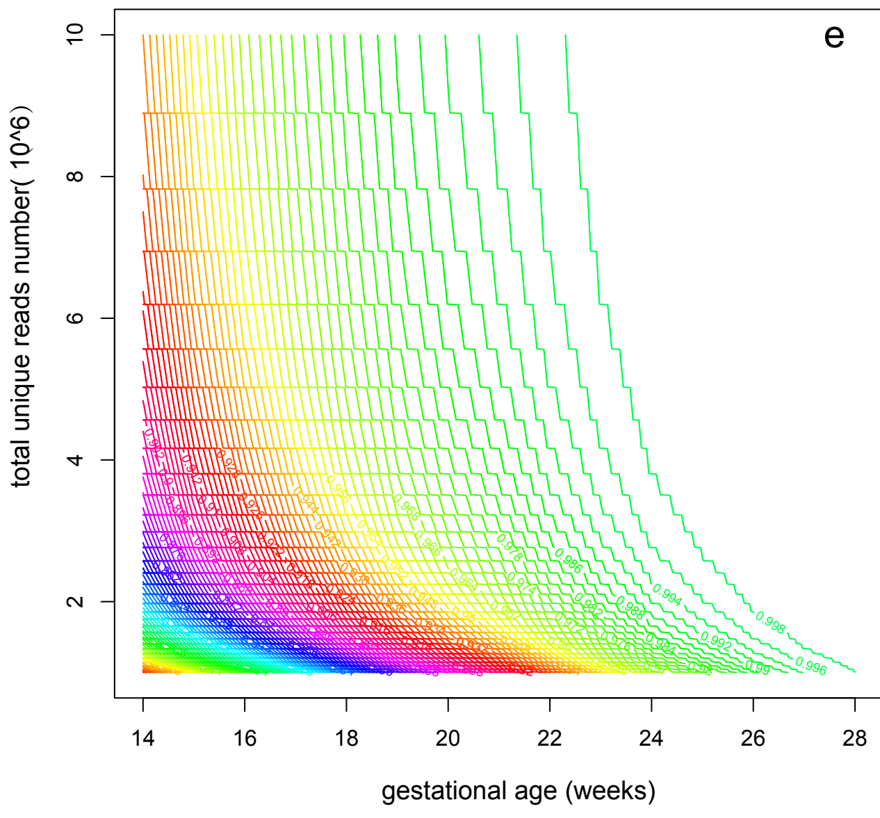
sensitivity of XXX or XO of chrX of female
