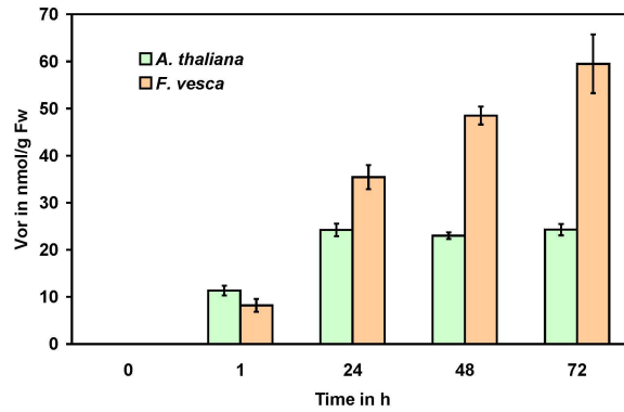
Figure S4. Uptake of voriconazole by A. thaliana and F. vesca . Three-week-old A. thaliana and F. vesca plants were transferred to liquid ATS media containing 25 \mu M voriconazole and incubated for the indicated time. Subsequently samples were taken and analyzed by HPLC-ESI-MS 2 . The average and standard deviation of three biological replicates is shown.
