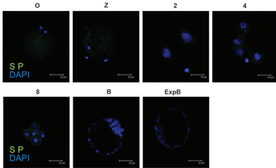
SUPPLEMENTARY FIG. S1. Control embryos corresponding to Fig. 2A [immunofluorescent detection of REX1 stained with A488 (green) in confocal sections]. Negative control embryos from the same experiment incubated without primary antibody (SP) and processed in parallel are labeled as follows: O, oocyte at metaphase II; Z, zygote; 2, 4, 8: 2-, 4-, 8-cell embryos; M, morula, B, blastocyst. Chromatin staining with DAPI is shown in blue. Scale bar=35 \mu m.
