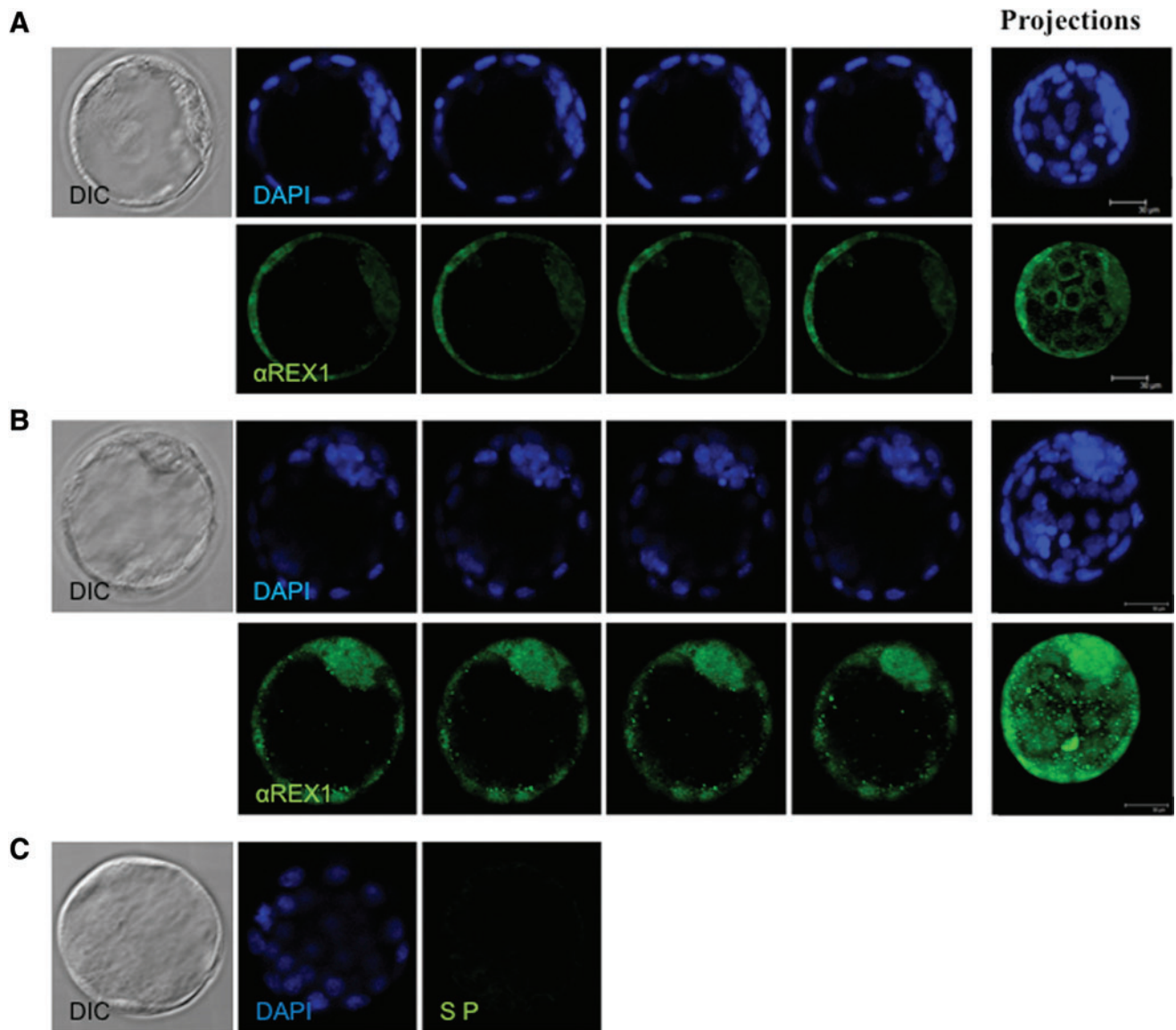
SUPPLEMENTARY FIG. S3. Detection of anti-REX1 immunoreactivity in late blastocysts (E4.5) in virtual confocal sections as in Fig. 2, except when indicated otherwise. Scale bar = 30 \mu m. DAPI staining and the corresponding \alpha REX1 immunoreactivity are shown in serial sections. (A) Example of perinuclear pattern. (B) Example of predominantly nuclear pattern. (C) Control embryo without primary antibody (SP).
