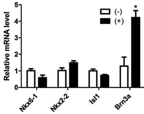
SUPPLEMENTARY FIG. S3. Expression of the midbrain basal plate markers at the end of the 5-stage dopaminergic differentiation experiments with positive and negative outcome. Relative mRNA expression levels of Nkx6-1 , Nkx2-2 , Isl1 , and Brn3a in experiments with positive (+) and negative (-) outcome, presented as mean \pm SEM; n=3 ; * P<0.05 significantly different from (-) experiments by Student t -test.
