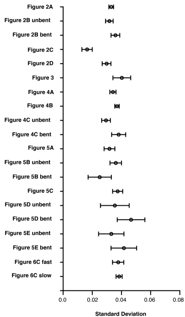
Figure S1. Plot of the standard deviations of the Gaussian fits as a measurement of their widths. The error bars represent the 95% confidence intervals. The free TATA-less DNA (Figure 2C) fits with a slightly narrower Gaussian; the widths of the remainder of the Gaussian fits are largely overlapping within their 95% confidence intervals.
