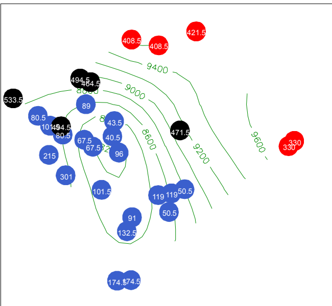
Cobalt
