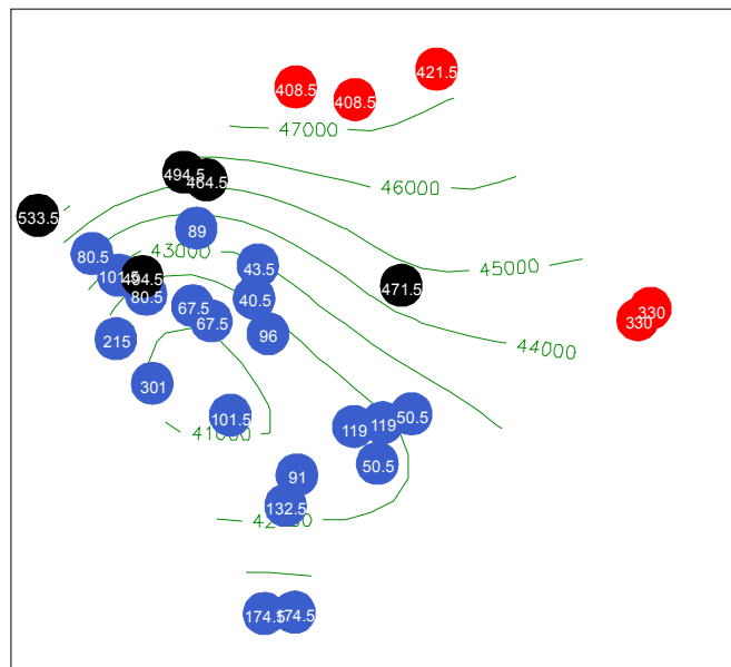
Iron
