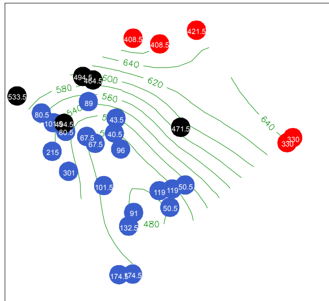
Carbon
