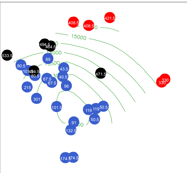
Magnesium
