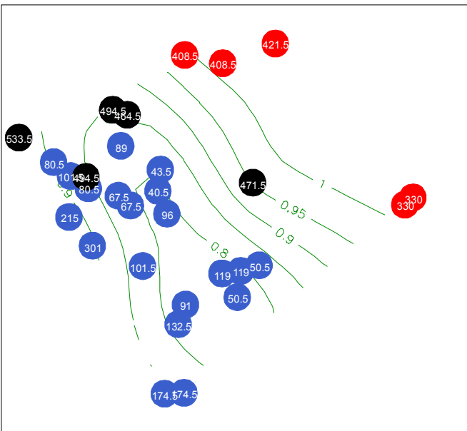
Thallium
