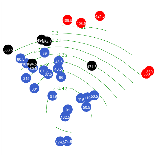
Nitrogen
