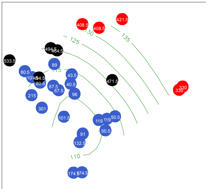
Vanadium
