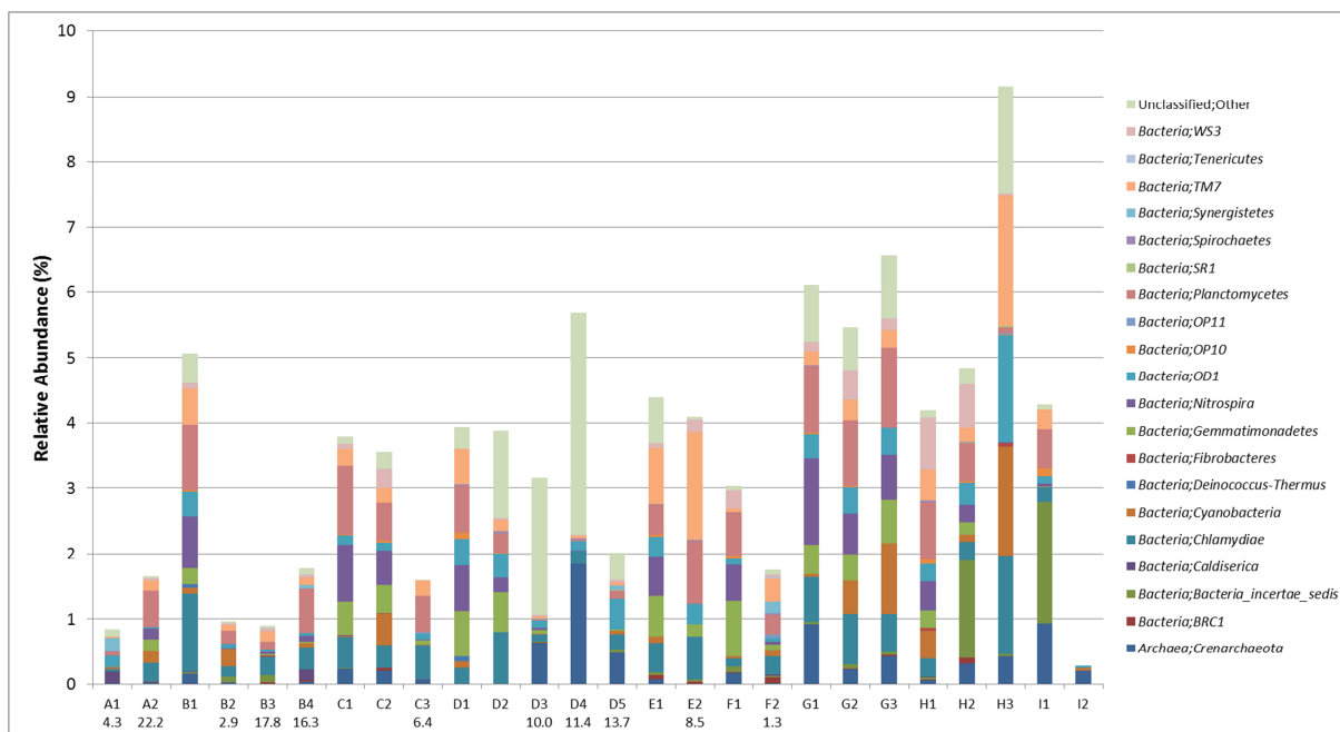
Figure S1. Relative abundance of minor microbial phyla (<1% of average abundance for the total pyrosequencing data set). Values below sample names indicate contamination as g TPH/kg soil.
