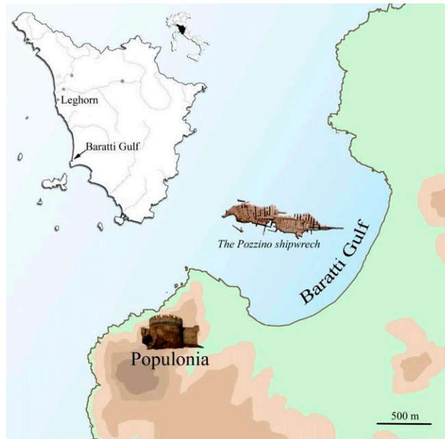
Fig. S1. Baratti Gulf near Populonia (Tuscany, Italy), where the Pozzino shipwreck was discovered.
