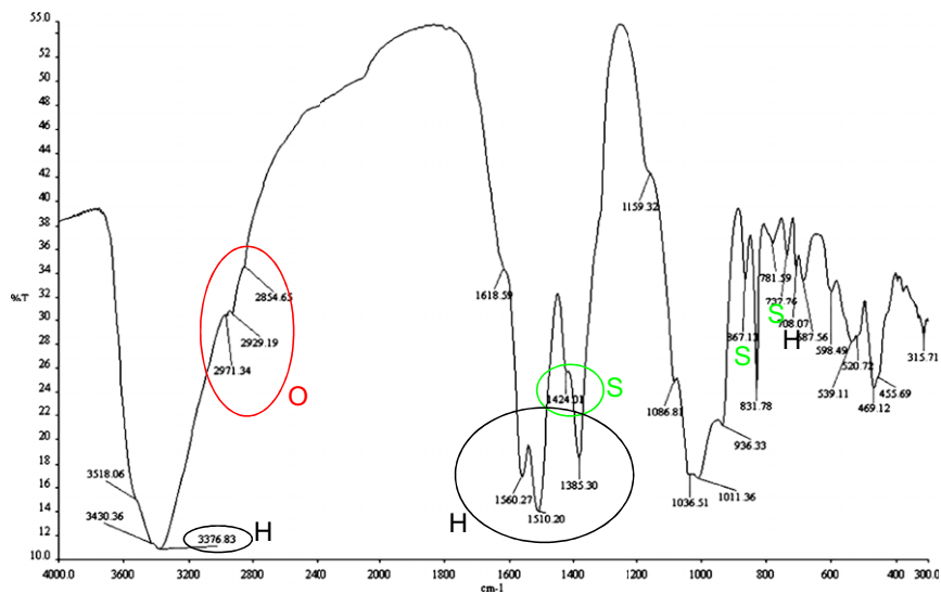
Fig. S2. FTIR spectrum of a subsample collected from the Pozzino tablet. H, hydrozincite; O, organic compounds; S, smithsonite.
