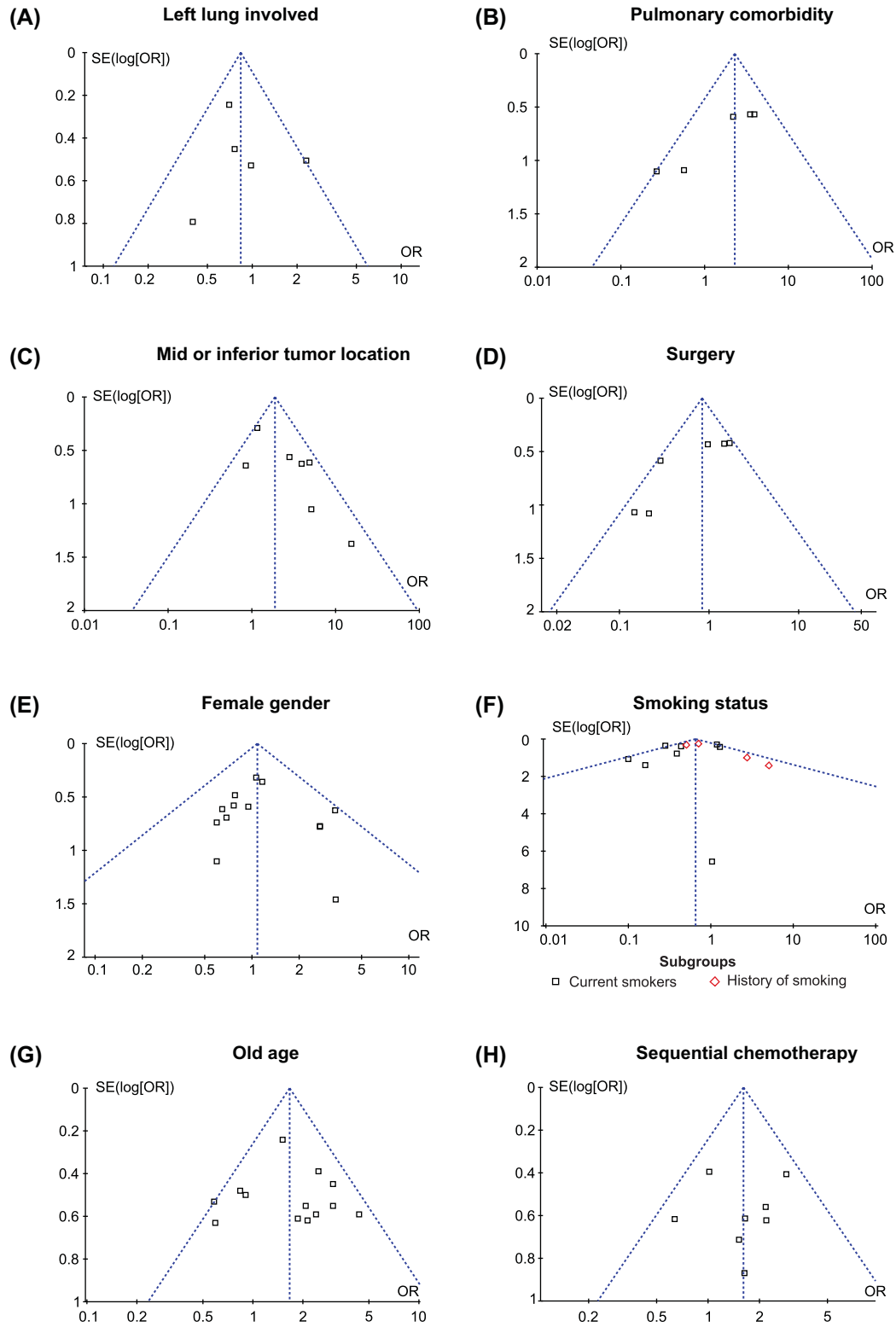
Supplementary Figure 1. Funnel plots corresponding to the pooled analysis in Figure 1.
