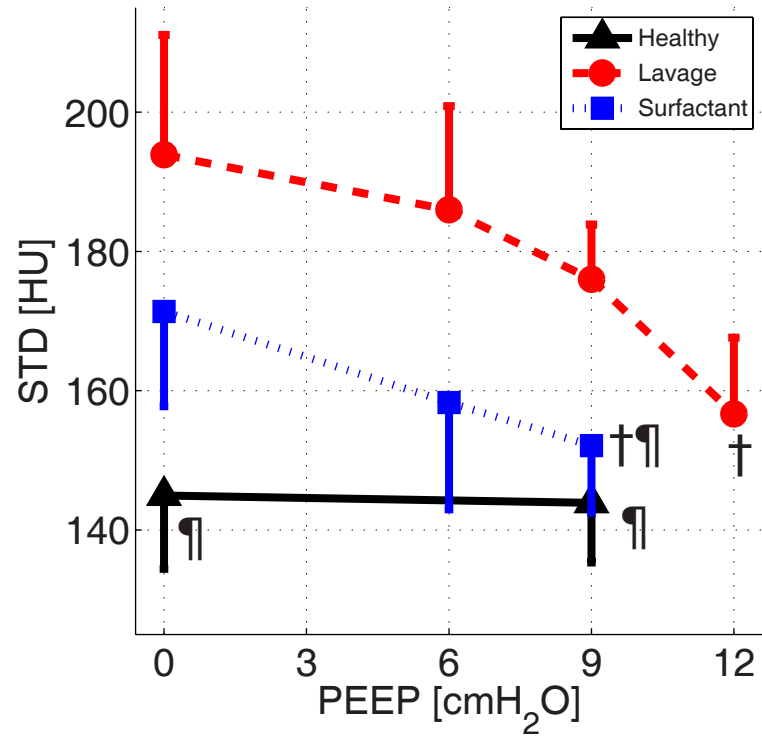
CT Density
