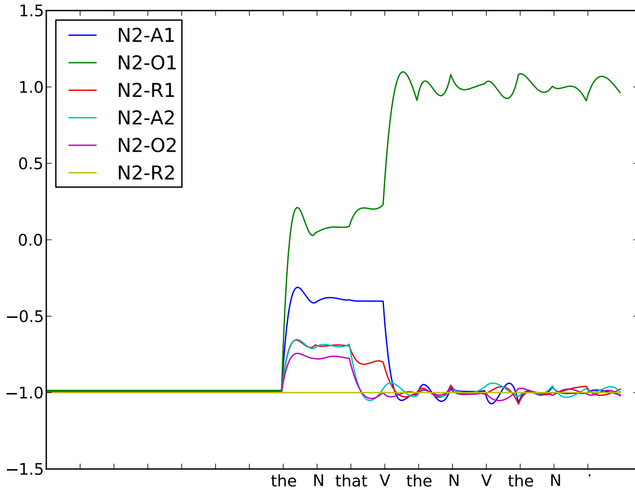
Sentence 20: 'the N that V the N V the N .'
