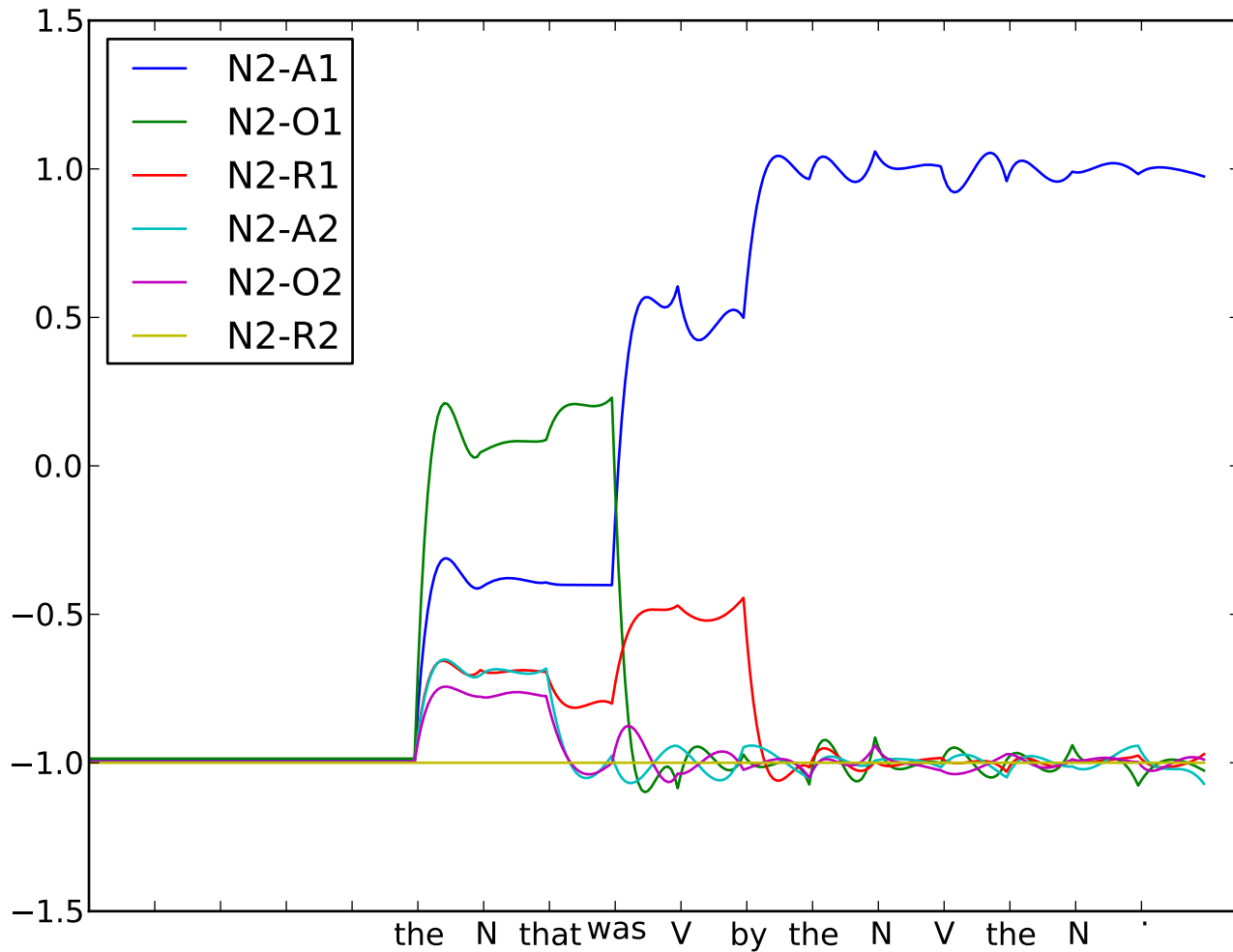
Sentence 24: 'the N that was V by the N V the N .'
