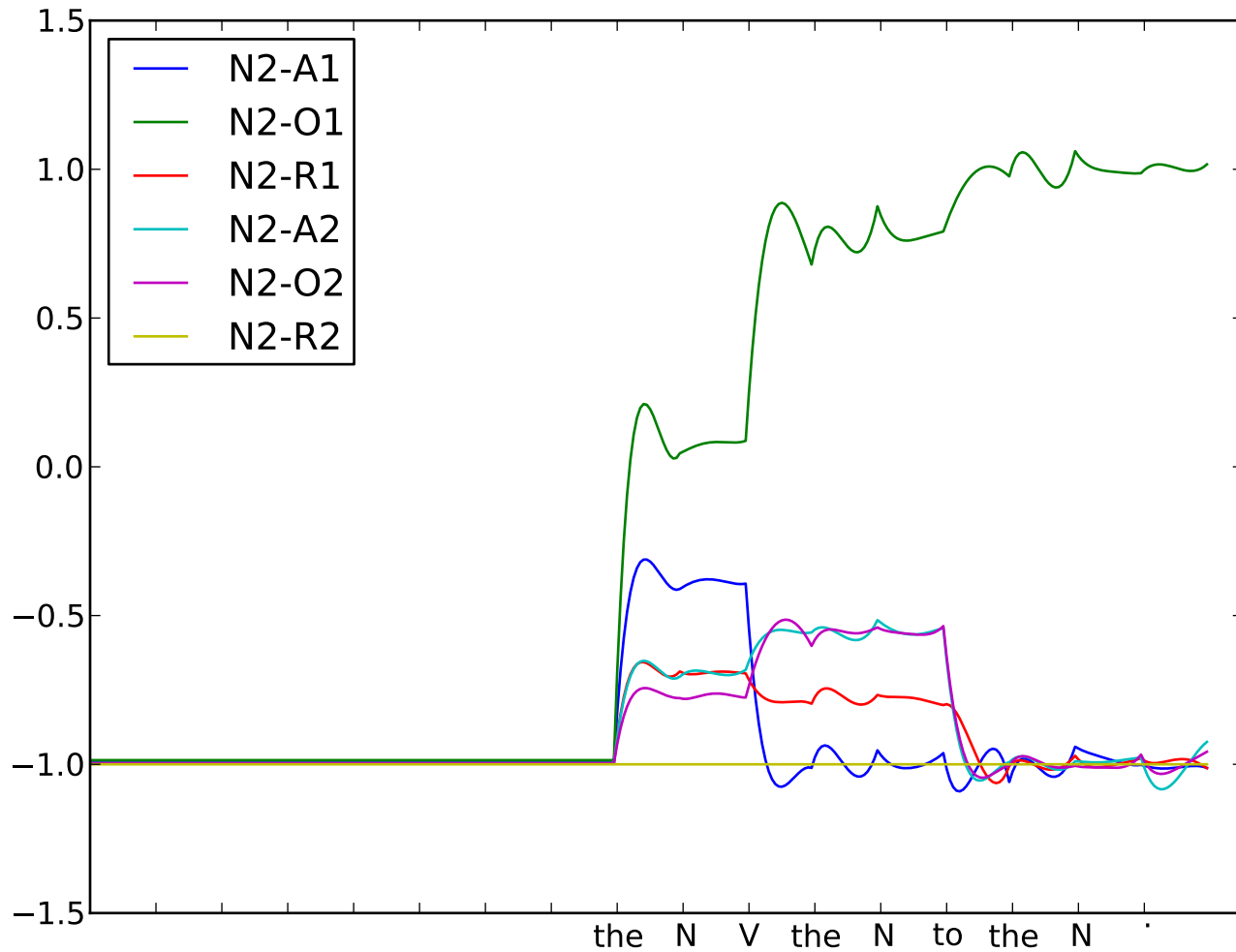
Sentence 17: 'the N V the N to the N .'
