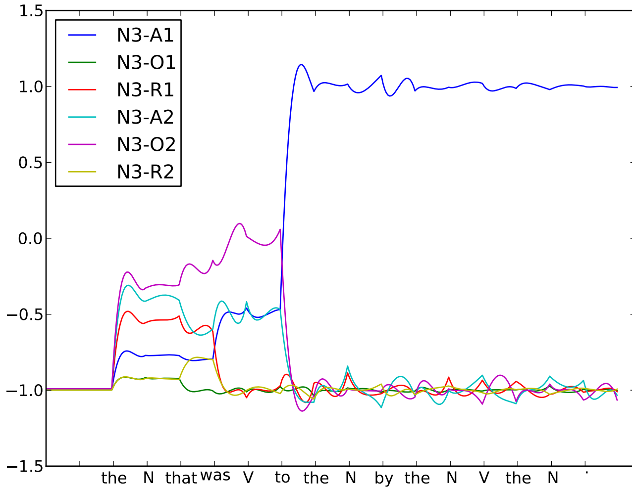
Sentence 38: 'the N that was V to the N by the N V the N .'
