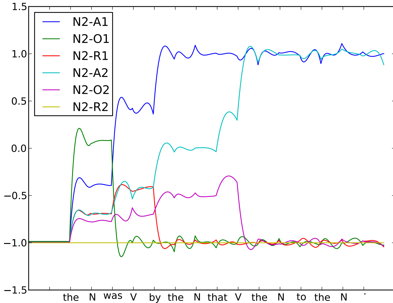
Sentence 35: 'the N was V by the N that V the N to the N .'
