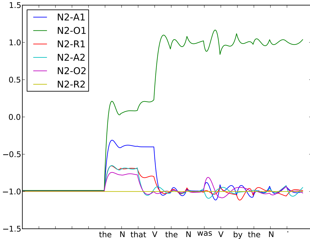
Sentence 22: 'the N that V the N was V by the N .'
