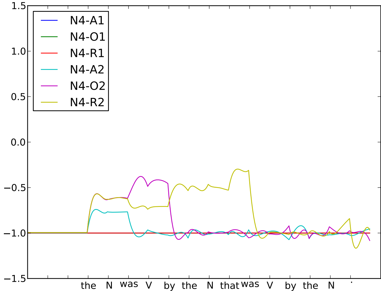
Sentence 25: 'the N was V by the N that was V by the N . '
