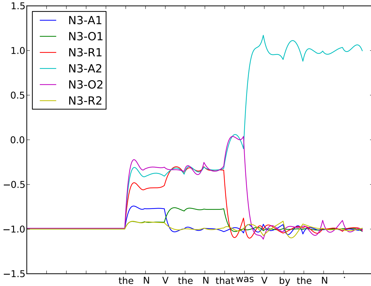
Sentence 27: 'the N V the N that was V by the N .'
