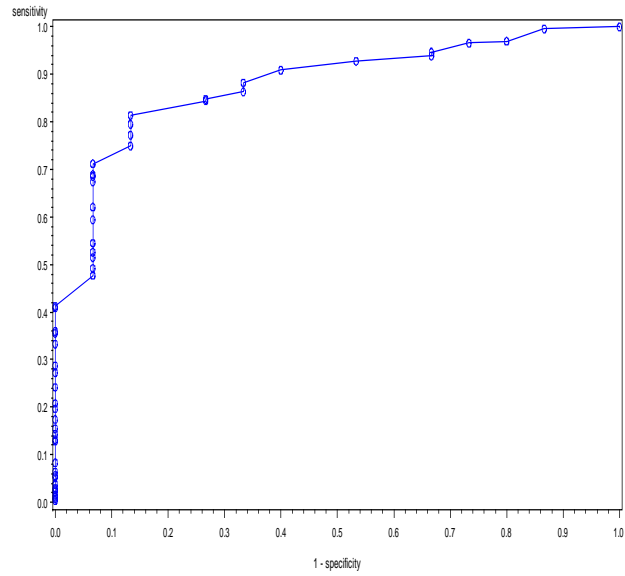
ROC for MSD predicting motor <70
