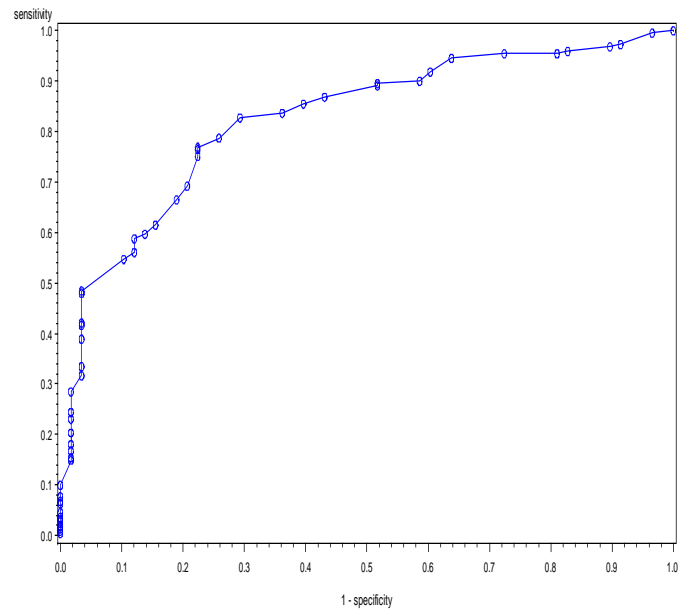
ROC for MSD predicting motor <85
