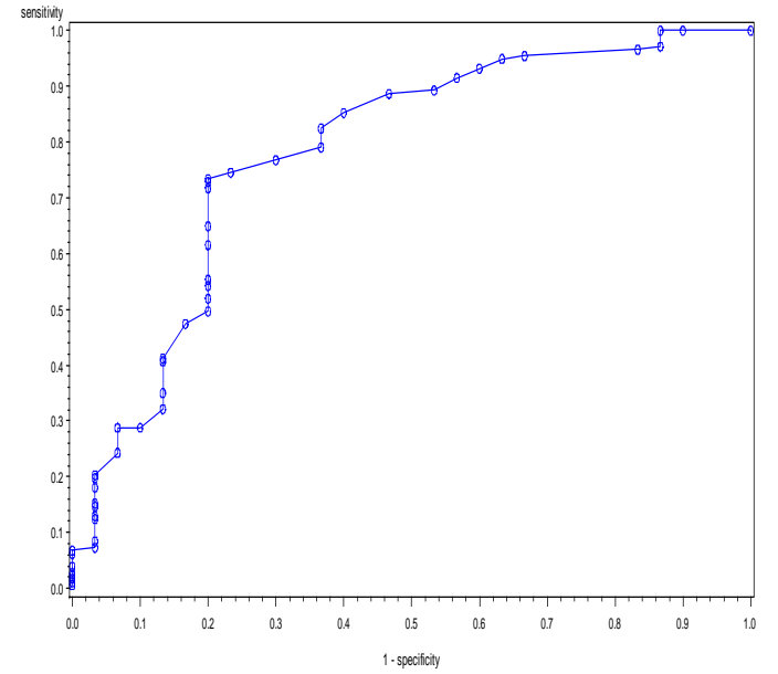
ROC for MSD predicting cognitive <85
