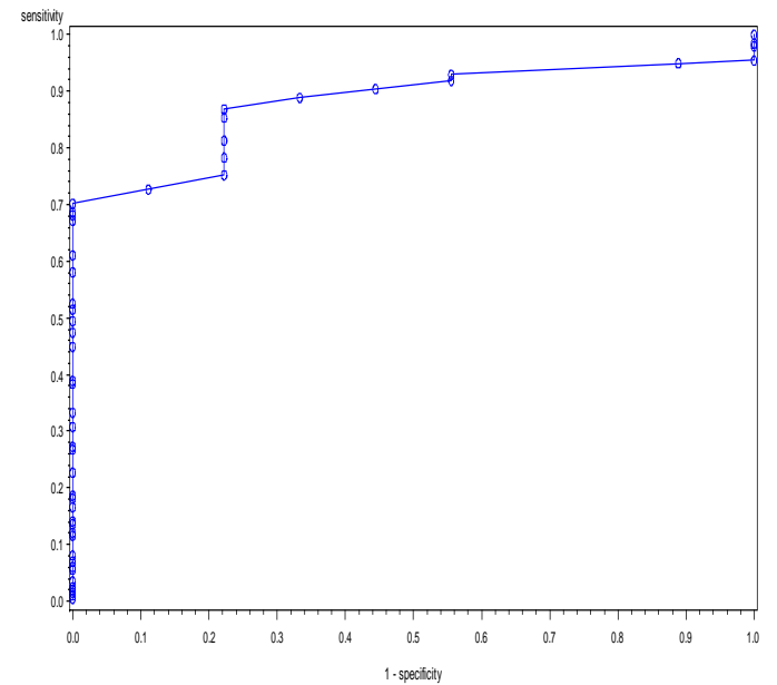
ROC for MSD predicting cognitive <70
