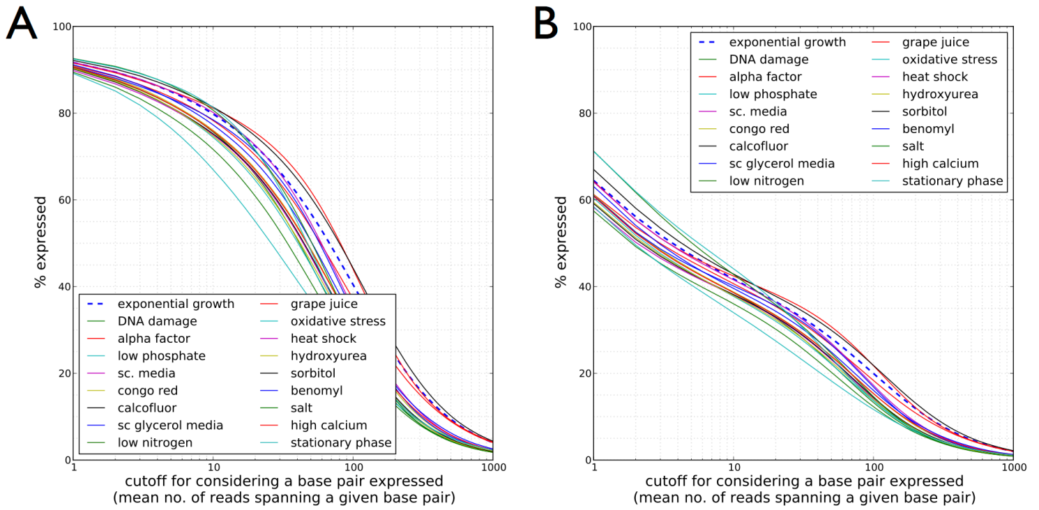
Figure S1 Read coverage of the yeast genome. Shows the percentage of the genome covered to a given read depth (or more). On the left are the percentages for transcription coming off either the plus or minus strand at any given locus, and the right shows percentages for the 24 Mb genome ( i.e. treating the plus and minus strand separately).
