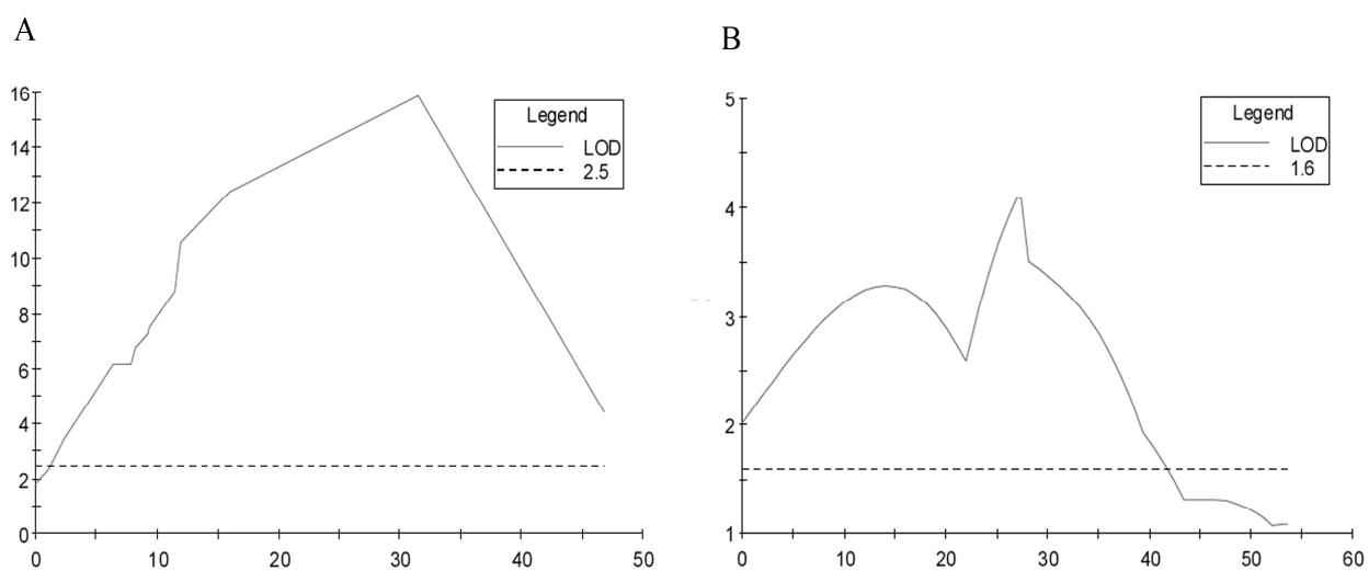
Figure S3. Mapping of sex determination loci in LG1(A) and LG22(B) The dotted lines indicate the significance thresholds of the LOD score in linkage groups.
