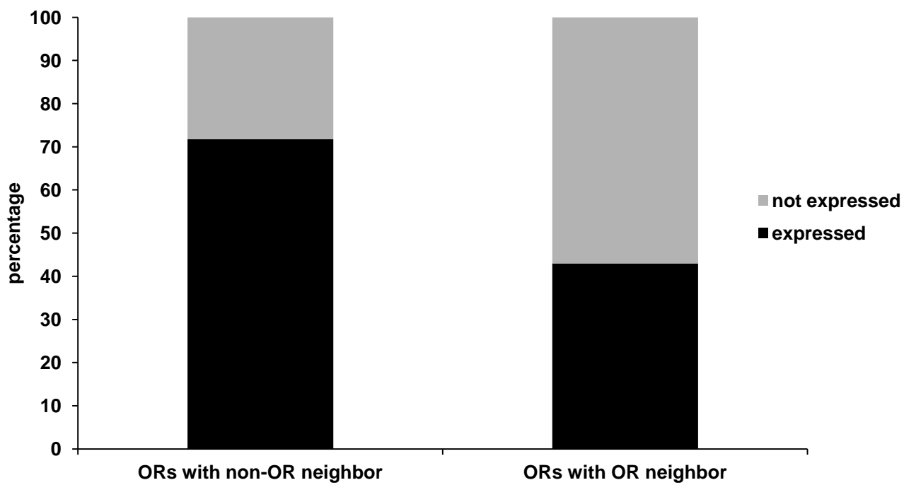
Dependence of OR expression on the genomic neighborhood
