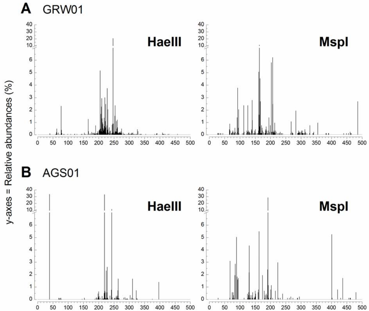
Figure AF4.1 – Examples of full digital T-RFLP profiles obtained with the restriction enzymes HaeIII and MspI for the samples GRW01 (A) and AGS01 (B).
