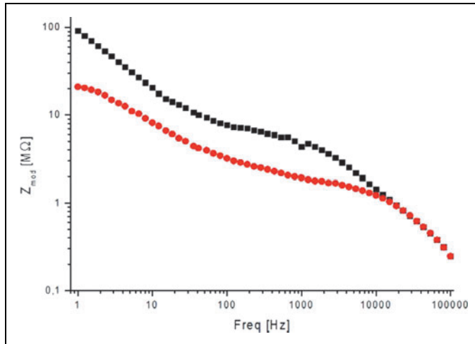
Supplementary Fig. S2. Typical impedance spectroscopic measurement of a single-spike microelectrode before (squares) and after (circle) chlorination. The modulus Z_{mod} measured at frequencies <10,000 Hz dropped down after chlorination protocol, showing a successful chlorination of the tip.
