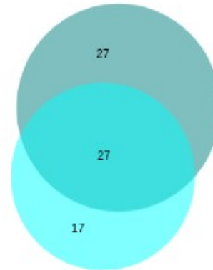
n=15, stepwise model
