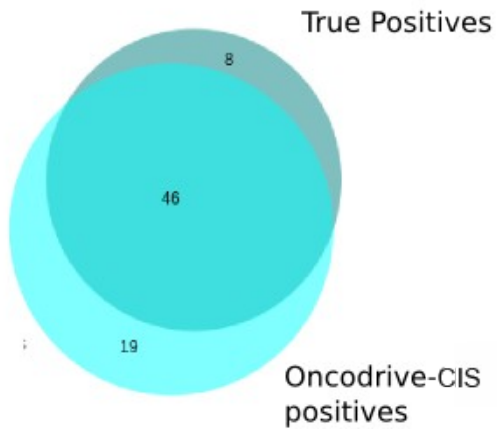
n=100, lineal model
