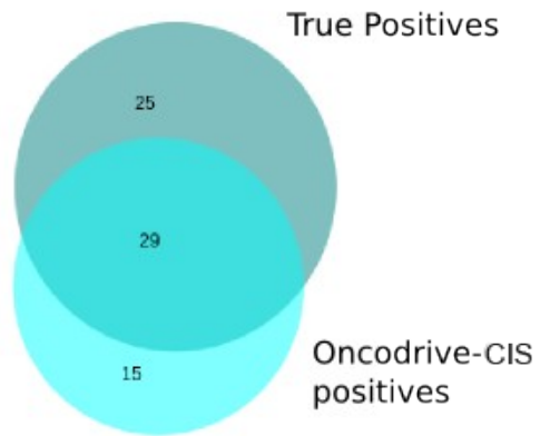
n=15, lineal model
