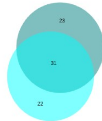
n=100, sigmoid model
