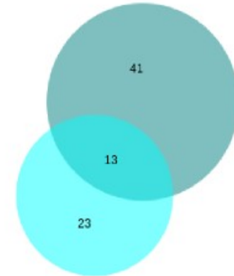
n=15, sigmoid model
