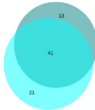
n=100, stepwise model
