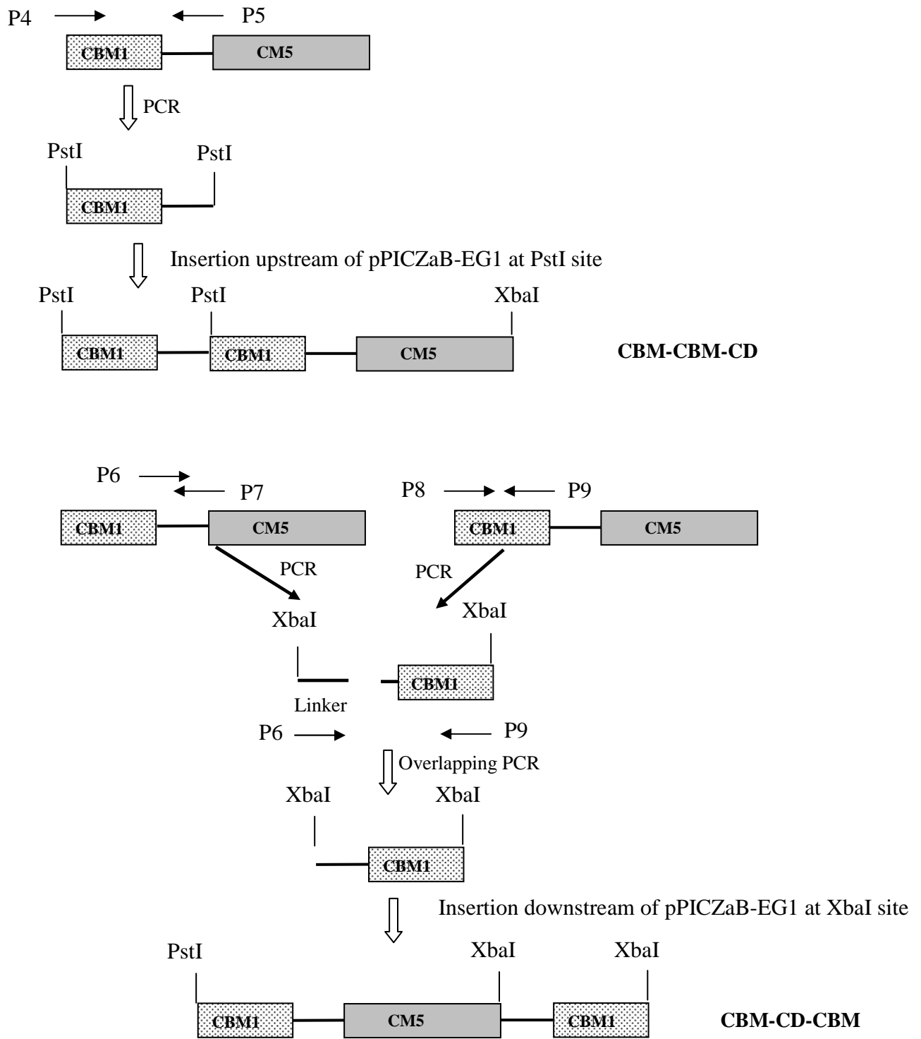
Fig.1S: Construction of pPICZaB-CBM-CBM-CD and pPICZaB-CBM-CD-CBM
