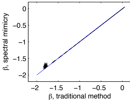
AR(1) model
