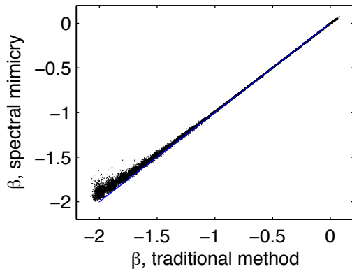
1/f model
