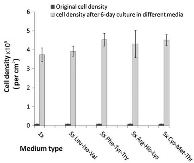
SUPPLEMENTARY FIG. S1. Essential amino acid concentrations up to five times physiological had no detrimental effect on viability or cell proliferation in monolayer culture over 6 days (mean \pm SD, n=5 ).
