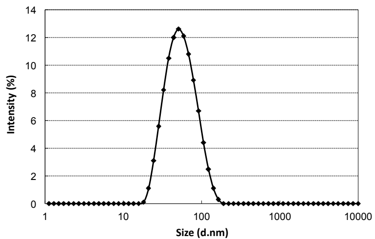
Figure S1 Size distribution of polyplex nanomicelle determined by dynamic light scattering (DLS).
