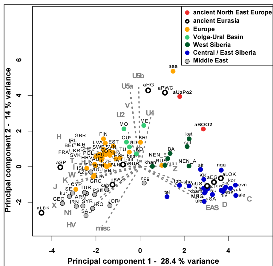
Figure S2. Principal Component Analysis of mtDNA haplogroup frequencies, non-redundant ancient haplotypes only. A. Recalculated frequencies. B. PCA plot. The first two dimensions account for 42.4% of the total variance. Grey arrows represent hg loading vectors, i.e., the contribution of each hg.
