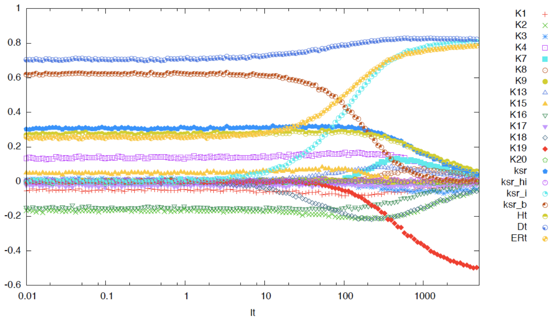
Supplementary Figure S1. The full spectrum of sensitivity of ER-dependent protein expression \bar{p} to the variation of the model parameters, calculated in the broad range of tamoxifen concentrations. Each colored label on the graph represents a value of PRCC coefficient between \bar{p} and corresponding parameter, calculated at certain fixed tamoxifen concentration It , as shown on the x axis.
