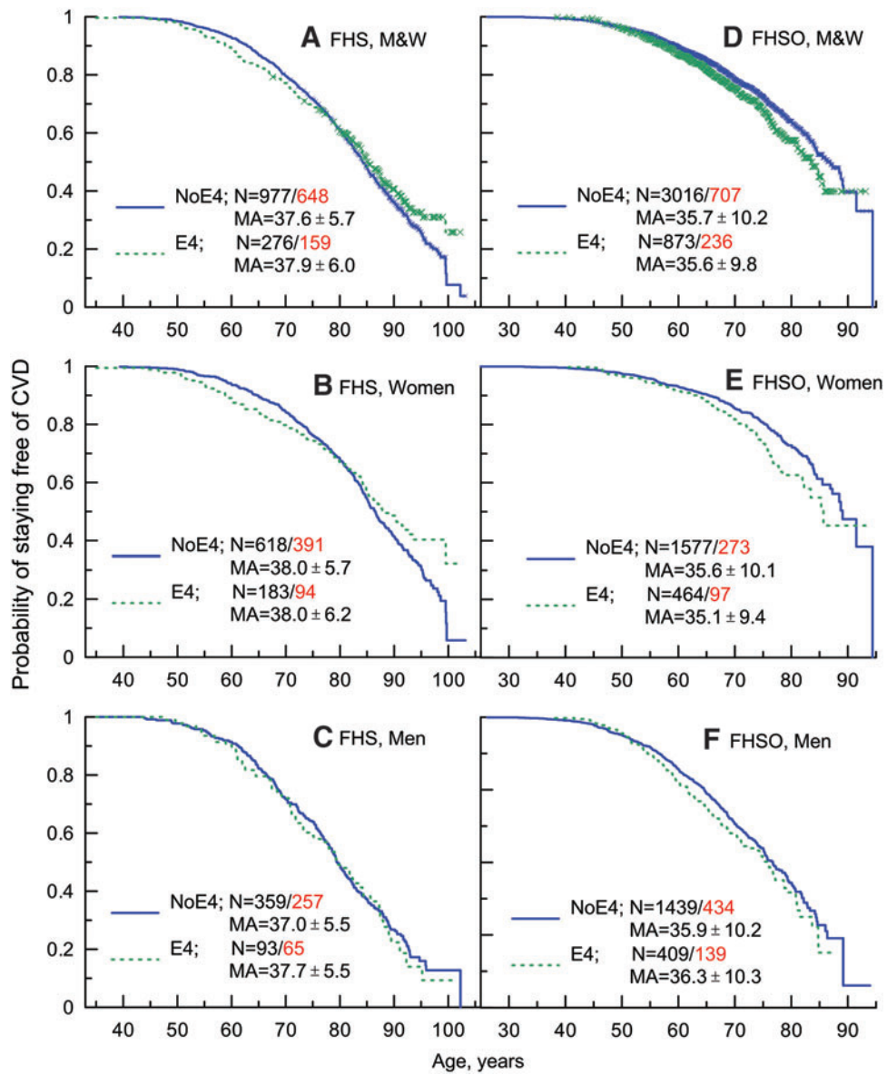
SUPPLEMENTARY FIG. S2. Kaplan–Meier age patterns of probability of staying free of cardiovascular disease (CVD) for (A–C) the Framingham Heart Study (FHS) original cohort participants and (D–F) the Framingham Heart Study offspring cohort (FHSO) participants carrying and not carrying the APOE e4 allele. N = m/k denotes the total number of carriers ( m ) and the number of events among them ( k ). MA, Mean age ± standard deviation.
