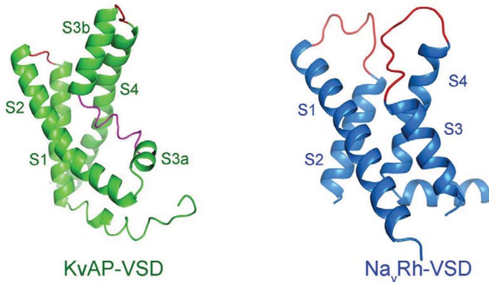
Figure S6. The distinct structural features of VSDs between KvAP and Na v Rh. KvAP contains an extended unwound region in the middle of the S3 segment. In contrast, flexible linkers exist between S1 and S2, S3 and S4 respectively in Na v Rh.
