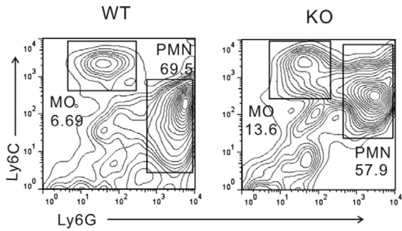
Figure S10 CD11b + cells in spleens of DA3-tumor bearing WT and CCL5 KO mice. MDSCs from DA3-tumor bearing WT and CCL5 KO mice were analyzed by using Ly6G and Ly6C mAbs.
