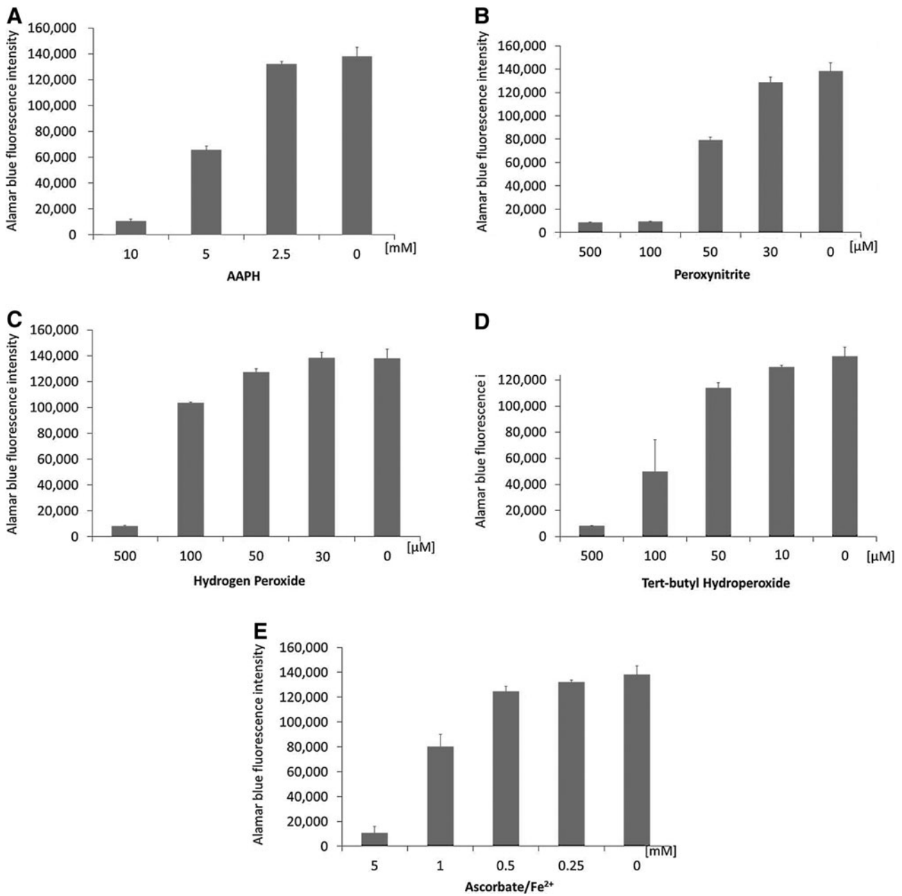
SUPPLEMENTARY FIG. S1. Effect of oxidizing agents on human mesenchymal stromal cell (hMSC) proliferation after 6 days. Effect of continuous exposure of 2,2'-azobis(2-amidino-propane) dihydrochloride (AAPH) (A), peroxynitrite (B), hydrogen peroxide (C), tert-butyl hydroperoxide (D), and the oxidizing system ascorbate/ \text{Fe}^{2+} (E).
