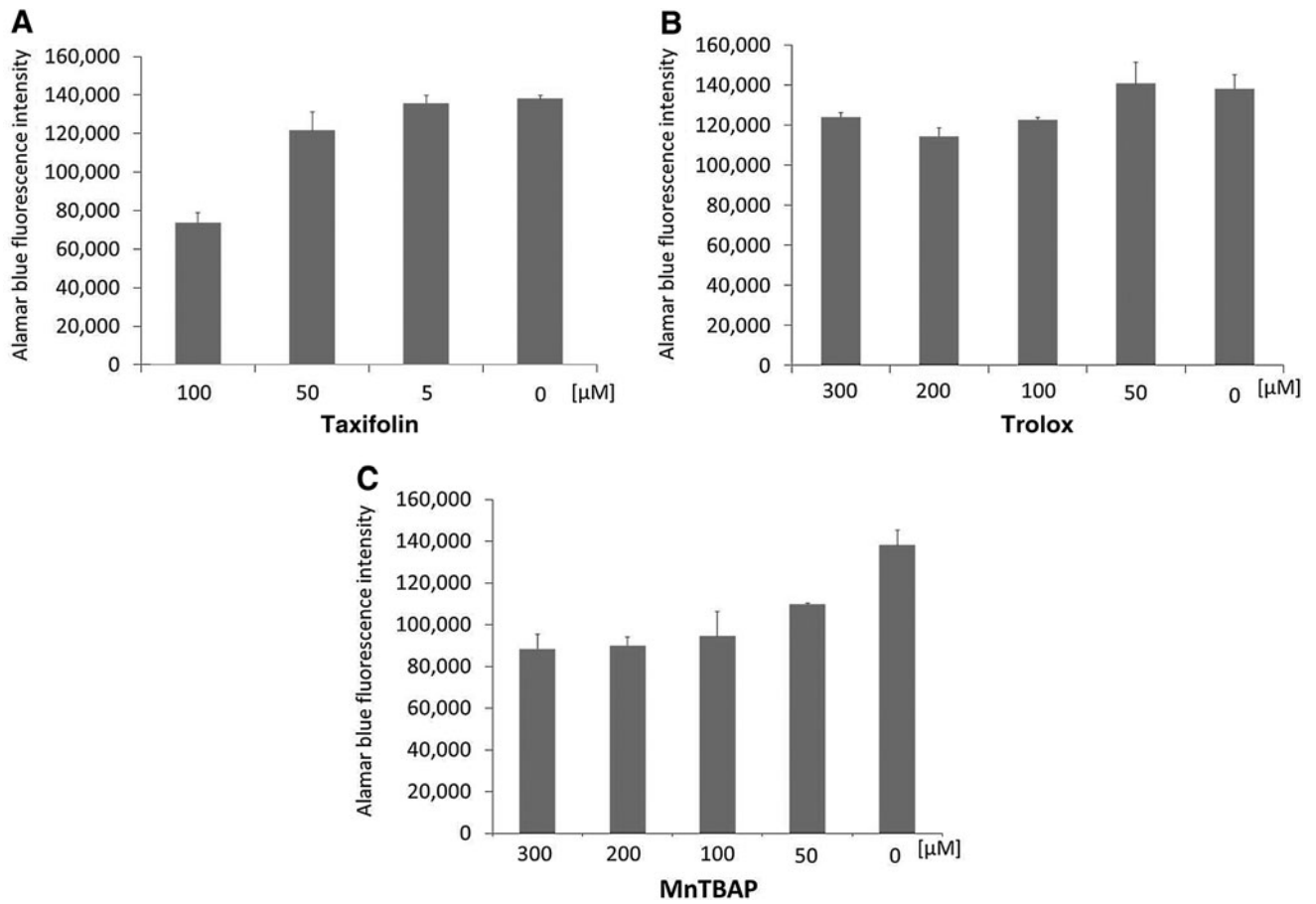
SUPPLEMENTARY FIG. S2. Effect of antioxidants/scavenger agents on hMSC proliferation after 6 days. Effect of continuous exposure of taxifolin (A), Trolox (B), manganese (III) tetrakis (4-benzoic acid) porphyrin chloride (MnTBAP) (C).
