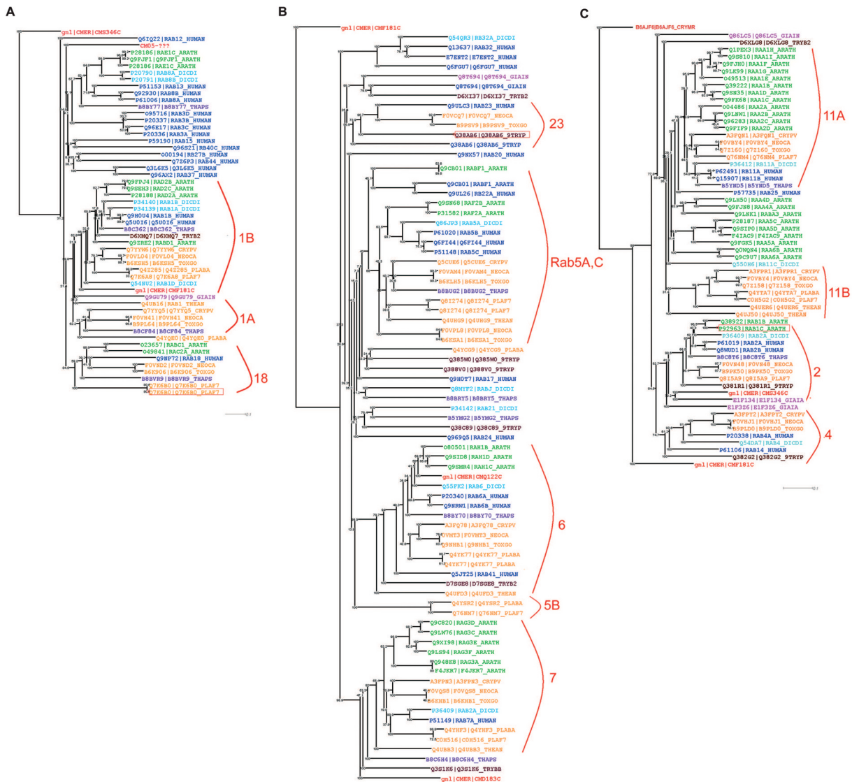
Figure S2. Rooted neighbour joining phylograms of 3 major clades (A,B,C) as described in Fig.1
