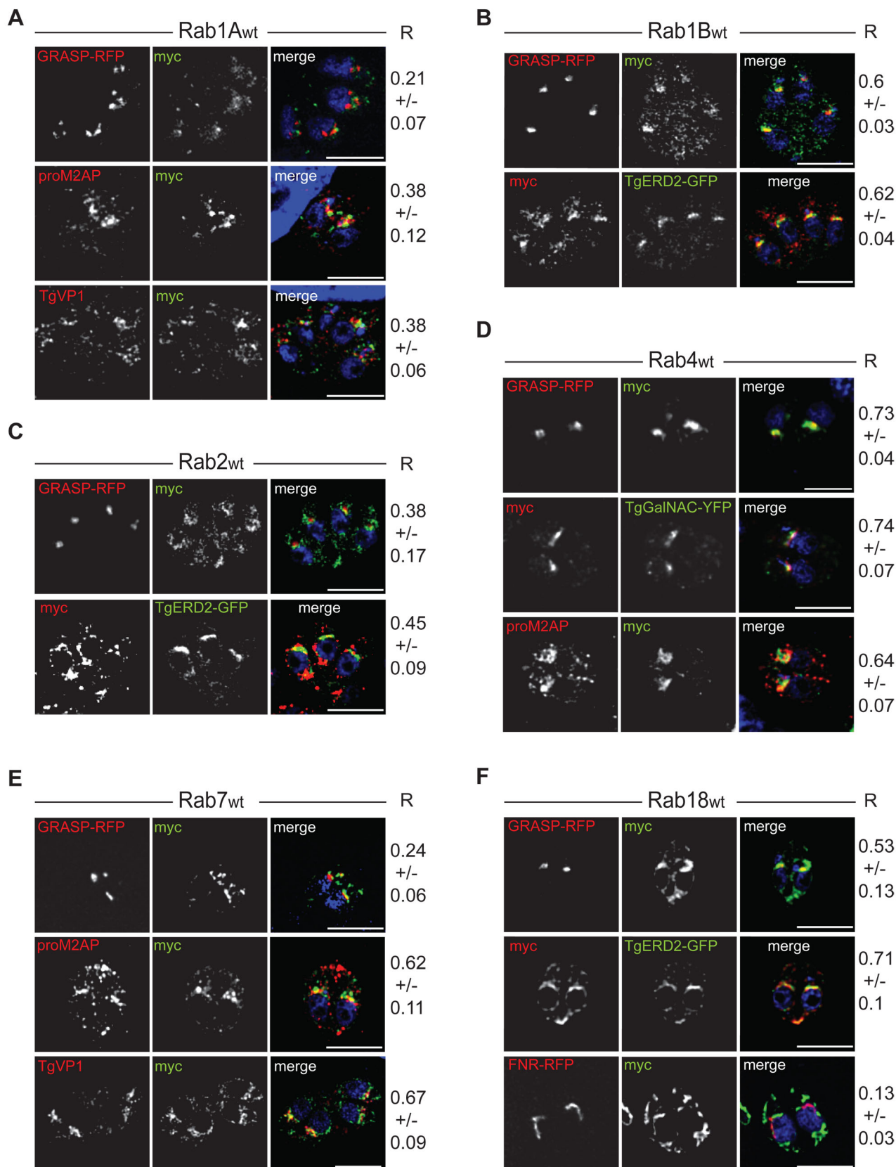
Figure S4. Localisation of Rab1A, Rab1B, Rab2, Rab4, Rab7 and Rab18
