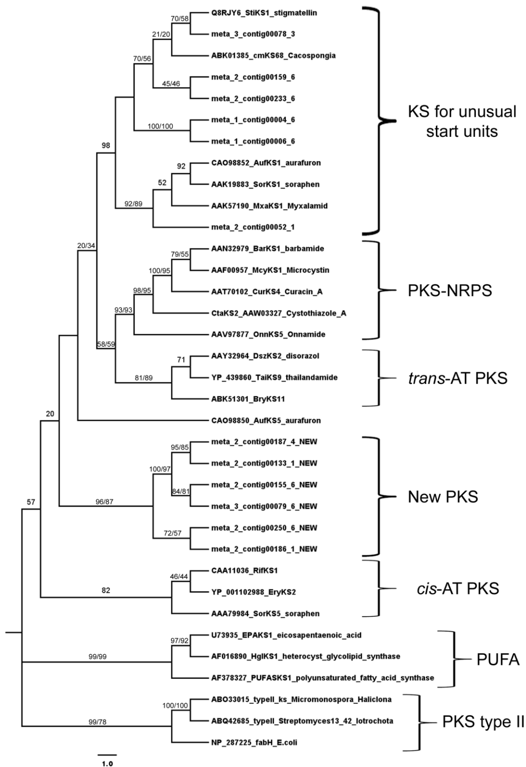
Supplementary Figure S3: Phylogenetic association between the novel A. brasiliensis -exclusive PKS group and PKSs of known function. The tree was constructed using Neighbor-Joining (NJ) and Maximum Likelihood (ML) methods. Numbers on the branches refer to NJ and ML bootstrap values (1,000 replicates and 100 replicates, respectively). The scale bar represents the substitutions/site.
