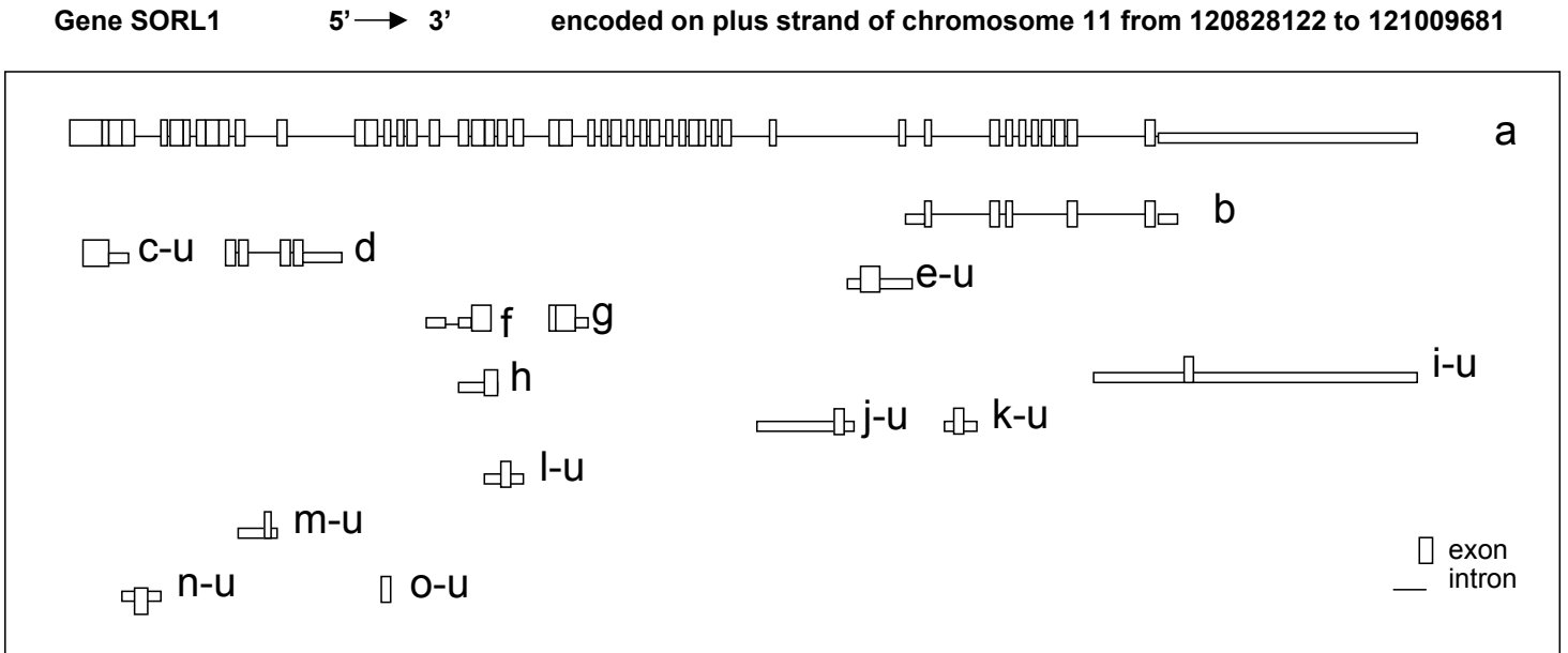
Fig. S1. A schematic view of the SORL1 locus. Protein sequences were analyzed in silico showing alternative protein variants (see Aceview annotations at www.ncbi.nlm.nih.gov/IEB/Research/Acembly ).
