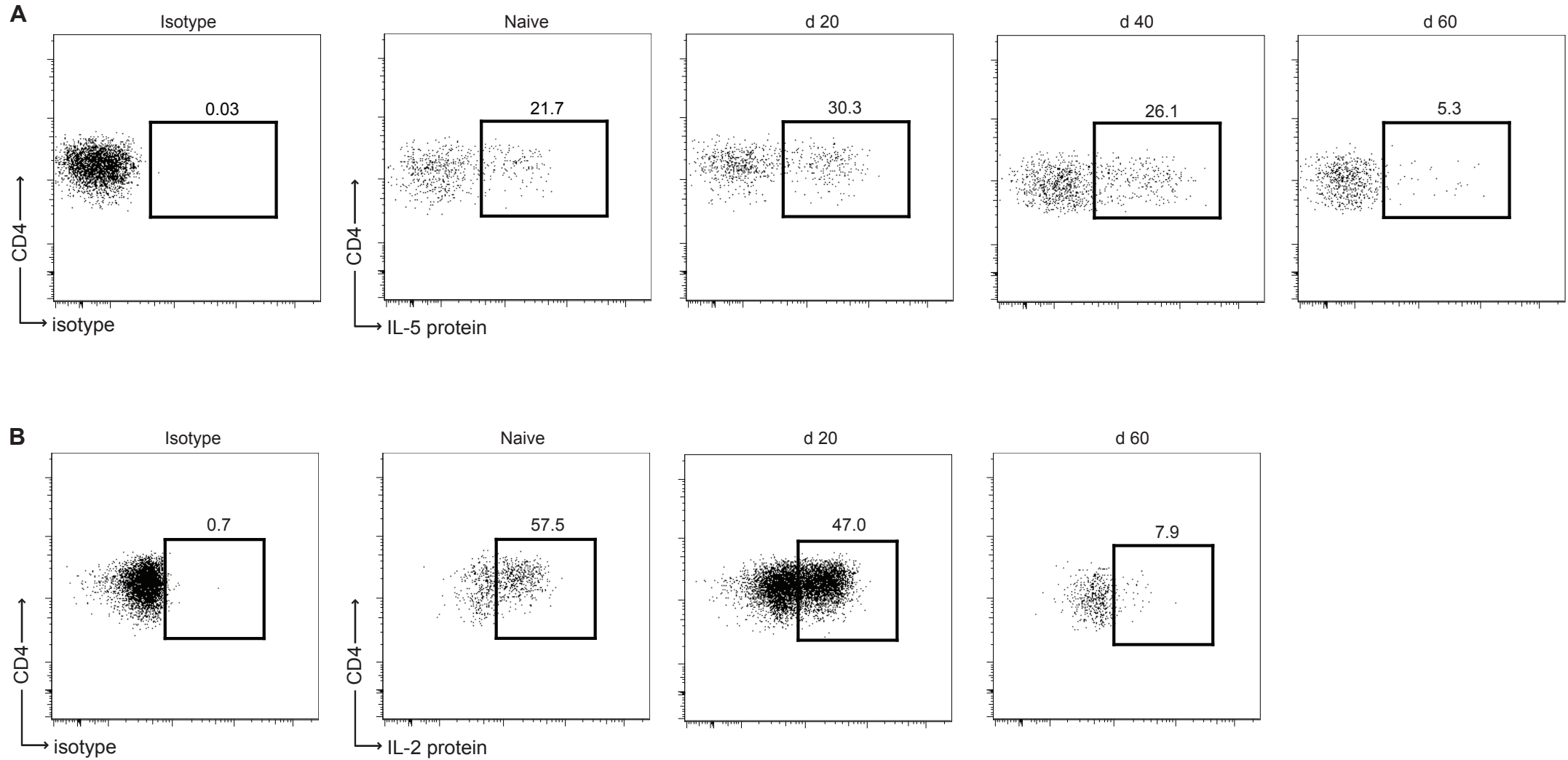
Figure S1. CD4 + Th2 cells lose their functional ability to produce IL-5 and IL-2 during L. sigmodontis infection. PC CD4 + T cells from naive and L. sigmodontis infected BALB/c IL-4gfp mice were analysed at d20, d40, and d60 pi for expression of GFP, IL-5 and IL-2. Representative flow plots showing expression of IL-5 (A) and IL-2 (B) by PC IL-4gfp + Th2 cells.
