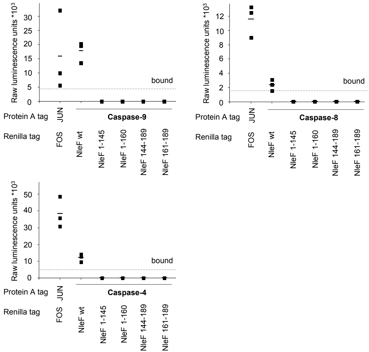
Figure S2. Interaction of Caspase-9, 8 and 4 with wild type and truncated versions of NleF. Numbers indicate amino acids present in the deleted versions. wt, wild type (amino acid 1 to 189).
