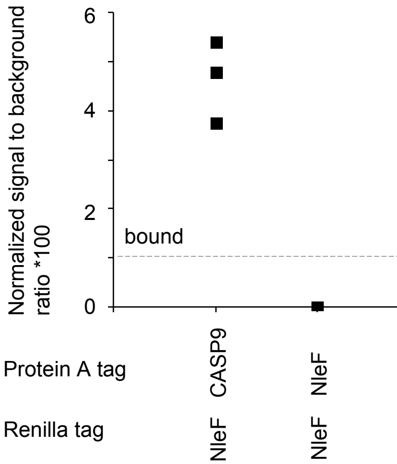
Figure S5. NleF is not a dimer. LUMIER assay of NleF against itself and against caspase-9.
