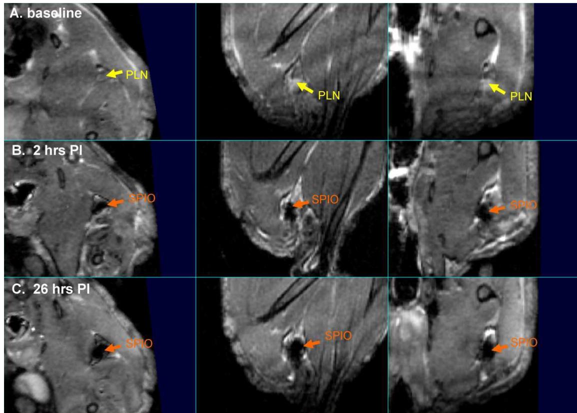
Figure S6. Magnified representative axial, sagittal and transverse MRI images of a xenograft mouse with SOR-C27-SPIO injection. (150\ \mu\text{m})^3 (magnified) axial, sagittal and transverse MRI images of a mouse with SOR-C27-SPIO injection showing (A) right popliteal lymph node (yellow arrow) at baseline scan, (B) SPIO is seen at 2 hours as indicated by dark signal void in the popliteal lymph node, and (C) SOR-C27-SPIO still remains at 26 hours post injection. Again the same trend was observed on the contralateral lymph node.
