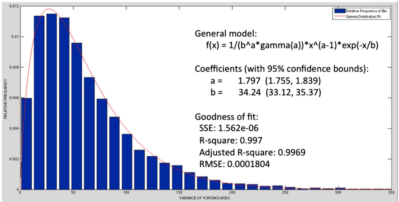
Fig. S1. Gamma distribution fit of the results of a simulation of a random cell with five organelles. This gamma distribution fits the simulation with an R^2 value of 0.997. RMSE, root mean square error; SSE sum of squared errors.
