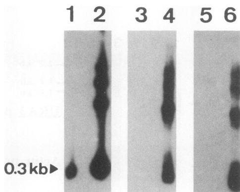
FIG. 5. Analysis of putative convergent transcripts downstream of the chromosomal ADHI , TRP1 , and TRP4 genes. Poly(A) + RNA of wild-type S. cerevisiae X2180-1A (lanes 1, 3, and 5) was probed with in vitro synthesized radiolabeled antisense RNA for putative convergent transcripts corresponding to the coding strand of the 3' end region of the ADHI (lane 1), TRP1 (lane 3), or TRP4 (lane 5) gene. For hybridization controls, the radiolabeled RNAs were hybridized to RNA from yeast strains containing the test plasmid with either the inserted ADHI (lane 2), TRP1 (lane 4), or TRP4 (lane 6) polyadenylation sites in reverse orientation.
