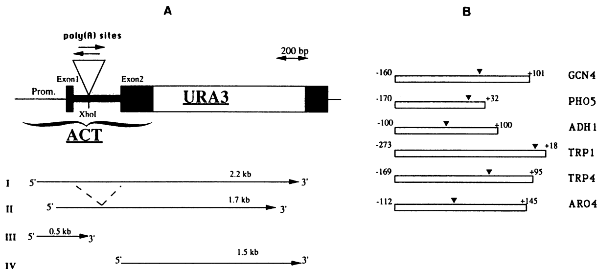
FIG. 1. Test system for polyadenylation sites. (A) Test gene on the 2\mu m-derived plasmid pME621. A part of the actin gene including the promoter, exon 1, intron, and a portion of exon 2 is fused to an URA3 cassette. The first six amino acids of the URA3 gene are missing, and the reading frame is maintained. DNA fragments containing the various polyadenylation sites are inserted in both orientations into the XhoI restriction site of the intron of the fusion gene. Expected transcripts are indicated below as follows: I, read-through transcription to the end of the URA3 gene results in a 2.2-kb transcript that is spliced to II, a 1.7-kb RNA; III, 3' end formation in the inserted fragment results in a truncated transcript of approximately 0.5 kb; IV, an additional 1.5-kb downstream transcript derives from a cryptic promoter and is discussed in the text. (B) Inserted DNA fragments containing the polyadenylation sites of six different yeast genes. All fragments were introduced in both orientations and contain DNA sequences from the end of the coding region of the corresponding gene to at least 18 bp downstream of the mapped 3' ends of the transcripts. The locations of the major poly(A) addition sites, as mapped at the chromosomal wild-type locus, are indicated by triangles, and the numbers represent the base pairs upstream and downstream of these sites.
