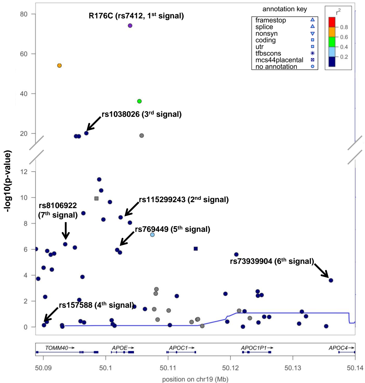
Figure S1. LDL-C locus TOMM40-APOE-APOC4 exhibited seven signals in African Americans. Each SNP was colored according to its LD ( r^2 ) in PAGE consortium with the strongest SNP rs7412 (R176C) colored in purple.
