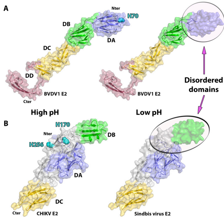
Figure S4. Structural Comparison of Pestivirus and Alphavirus E2 Glycoproteins at High and Low pH, Related to Figure 1
