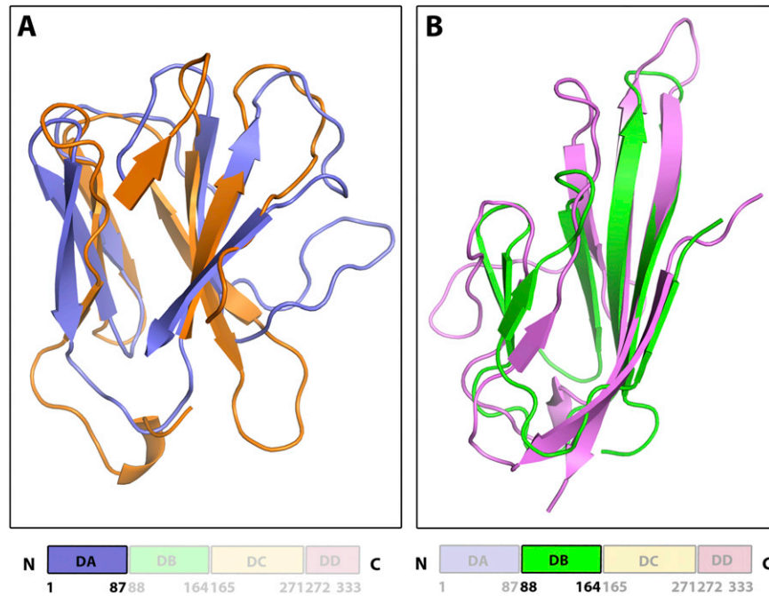
Figure S2. Domains DA and DB Have Ig-fold, Related to Figure 1
