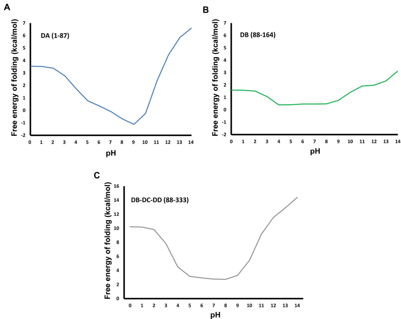
Figure S3. Stability of BVDV1 E2 Domains over pH, Related to Figure 1
